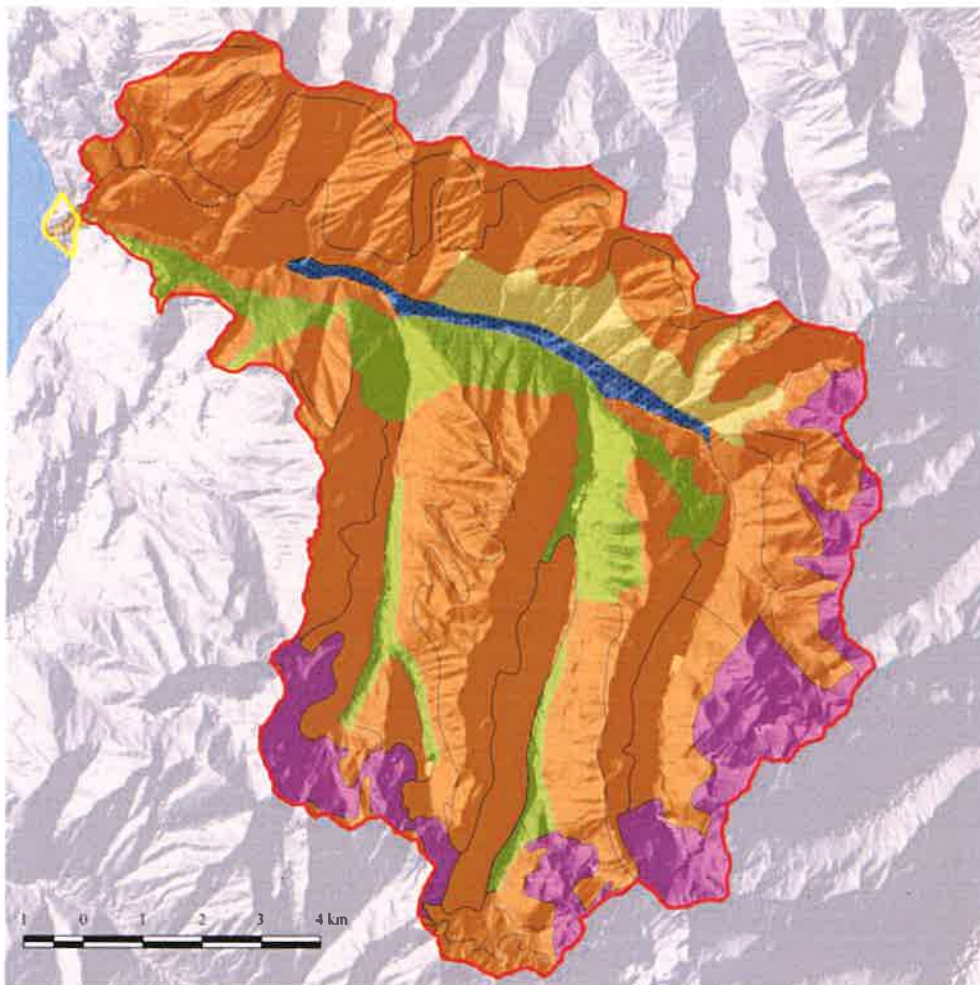
Silverton Watershed: Surficial Geology Map
