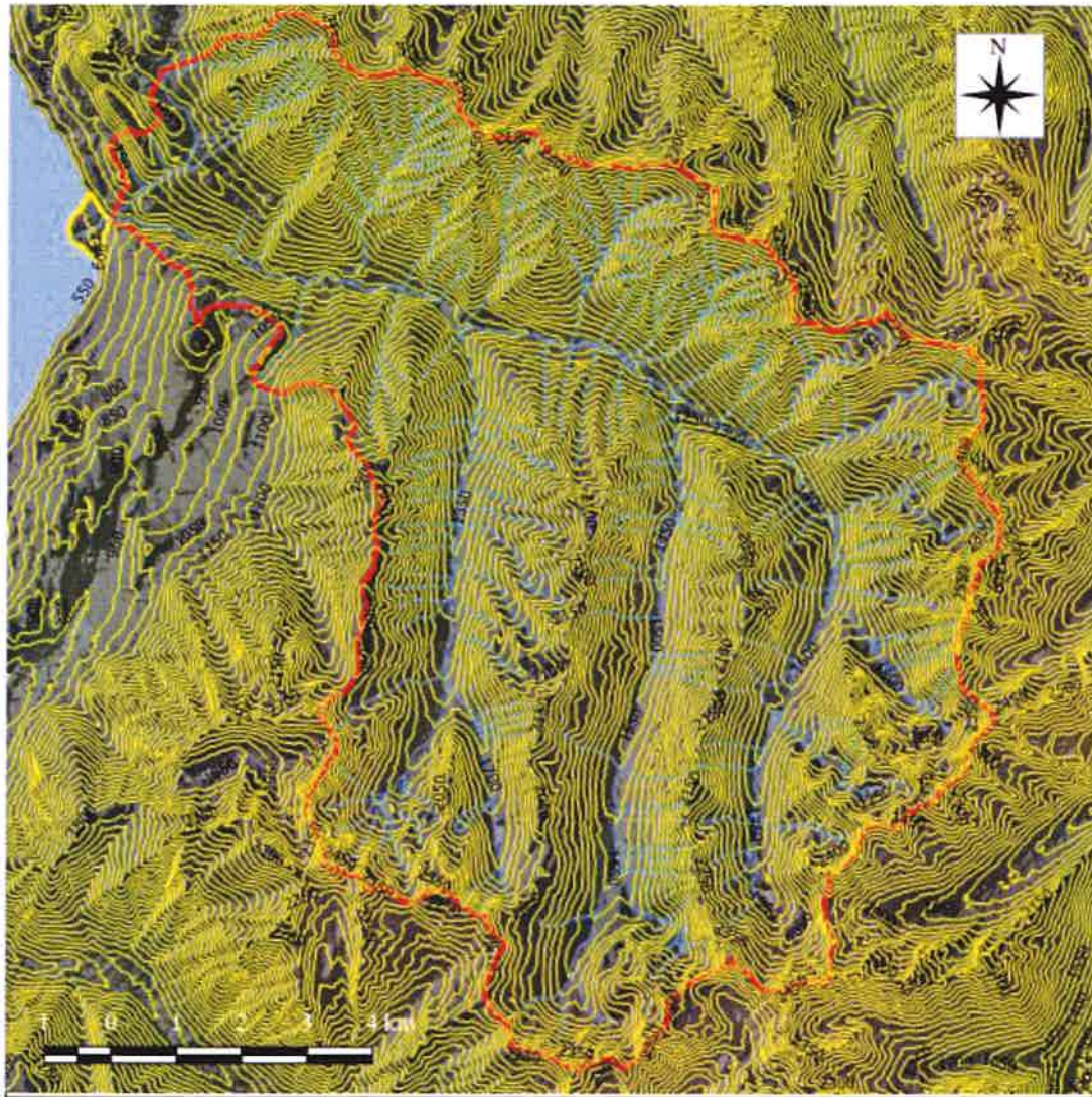
Silverton Watershed Topographic Map
