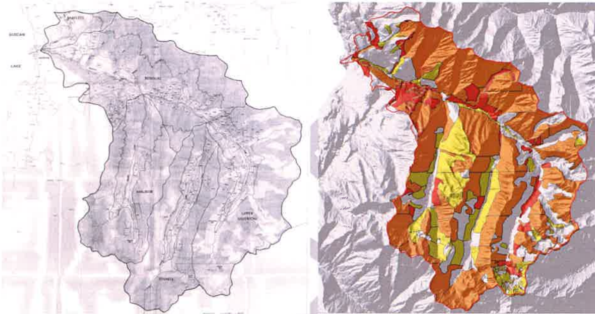
Map from Dobson IWAP Report
